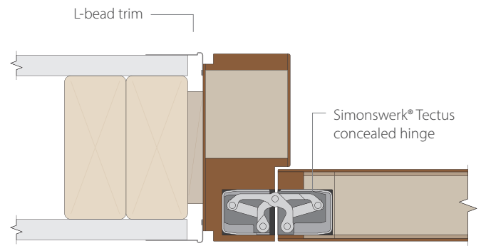
Jamb detail with L-bead trim and concealed hinge This option is available for 20-minute house-to-garage, natural wood door applications; minimum wall depth applies. Door closer required for self-closing requirements.
