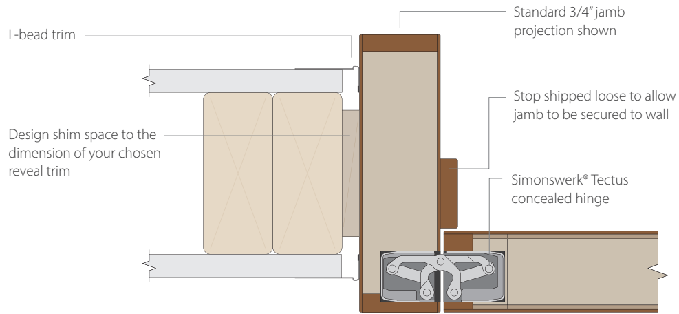
Jamb detail with L-reveal trim and concealed hinge
