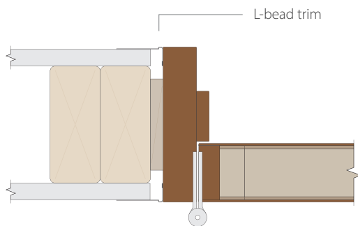
Jamb detail with L-bead trim and barrel hinge
