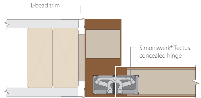
Jamb detail with L-bead trim and concealed hinge This option is available for 20-minute house-to-garage, natural wood door applications. Door closer required for self closing requirements.
