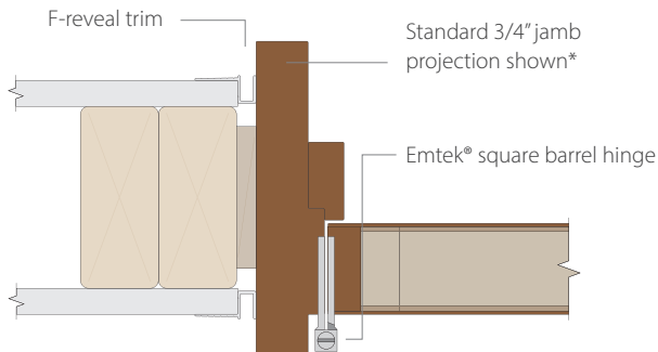
Jamb detail with F-reveal trim and barrel hinge
