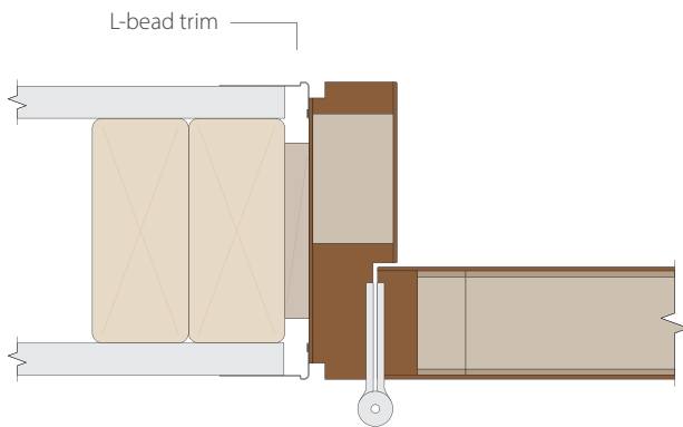
Jamb detail with L-bead trim and barrel hinge This option is available for 20-minute house-to-garage applications; minimum wall depth applies.
