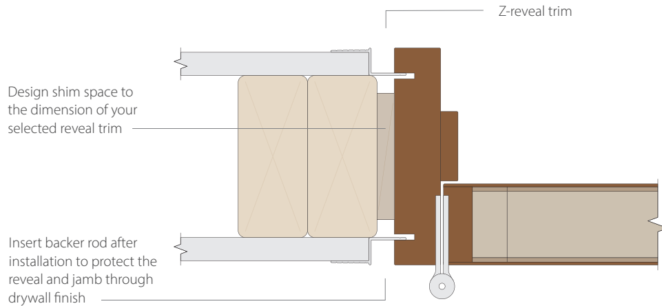
Jamb detail with Z-reveal trim and barrel hinge
