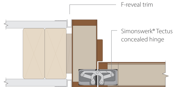
Jamb detail with F-reveal trim and concealed hinge
