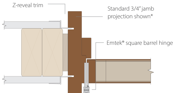
Jamb detail with Z-reveal trim and barrel hinge
