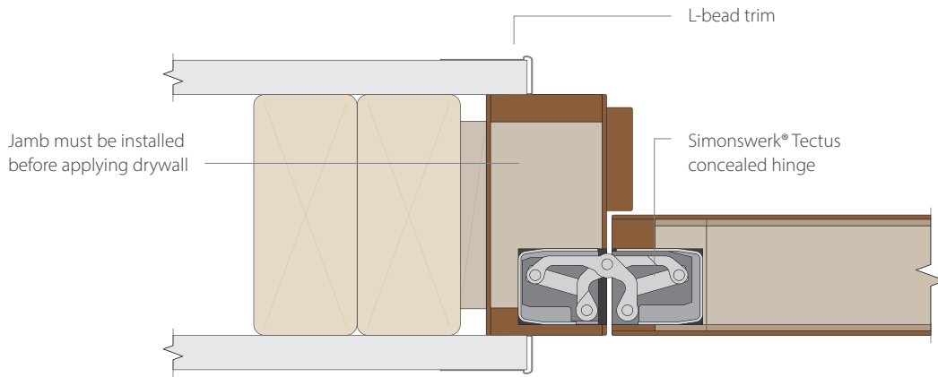
Jamb detail of drywall return jamb with concealed hinge
