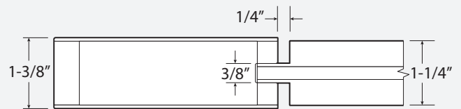
1-3/8" Profile with Square Stick (SS) sticking and Senior Flat (H) panel
