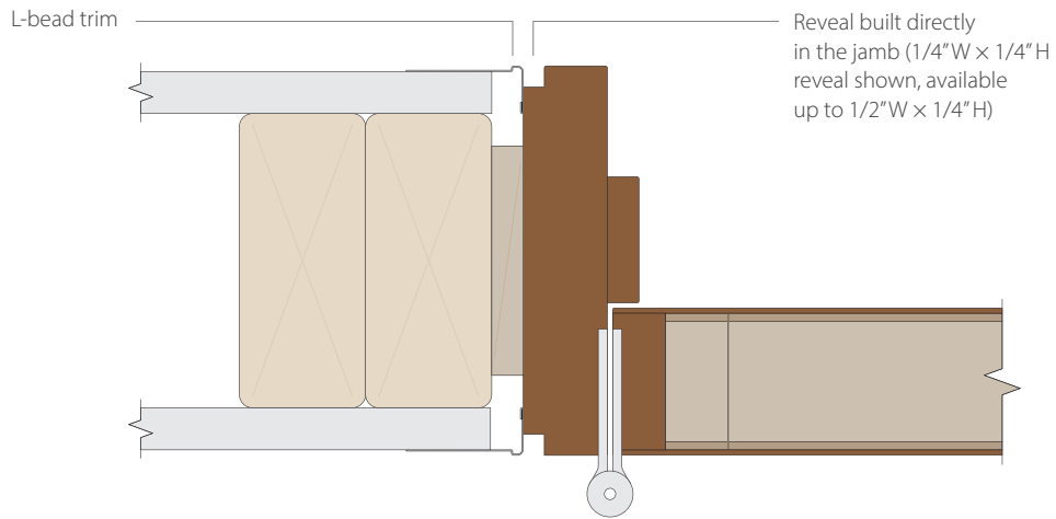
Jamb detail with L-bead trim and barrel hinge
