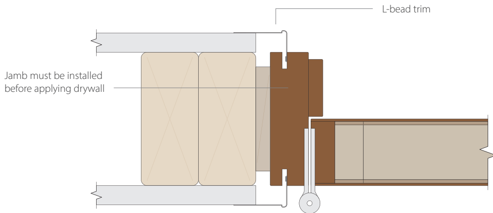
Jamb detail of drywall return jamb with barrel hinge
