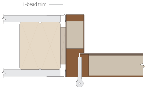
Jamb detail with L-bead trim and barrel hinge This option is available for 20-minute house-to-garage applications
