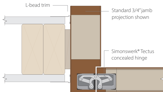
Jamb detail with L-bead trim and concealed hinge
