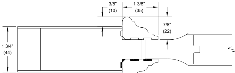
Bolection Moulding (BM)
