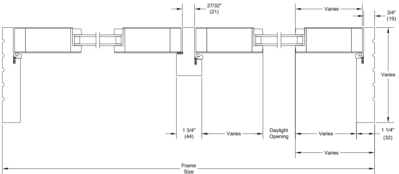
Jambs - Pair
