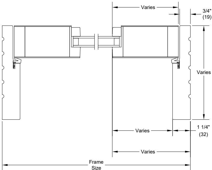
Jambs - Single
