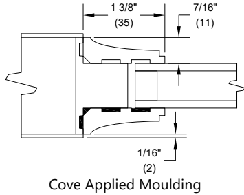
Cove Applied Moulding
