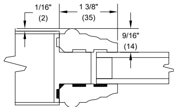
Low Profile Bolection Moulding (LP)
