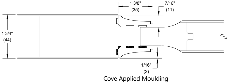
Cove Applied Moulding
