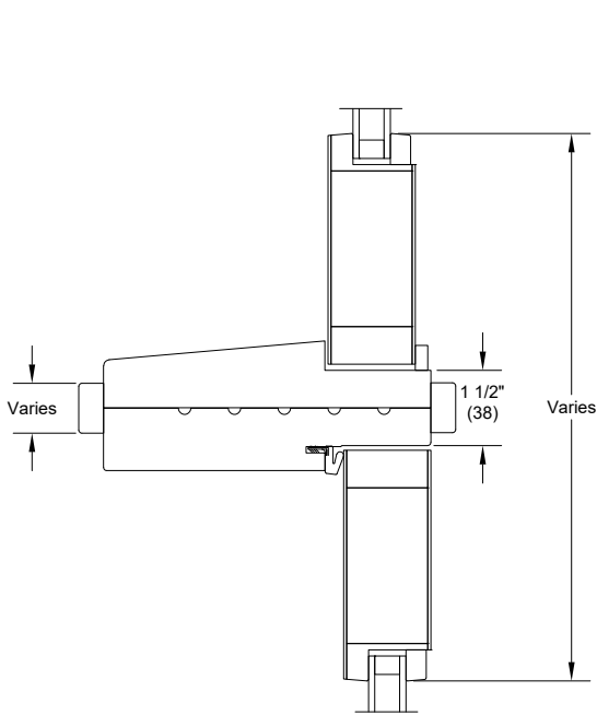
Direct Mull
