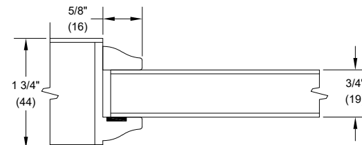
C - Flat
