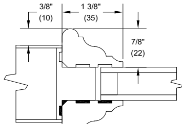
Bolection Moulding (BM)
