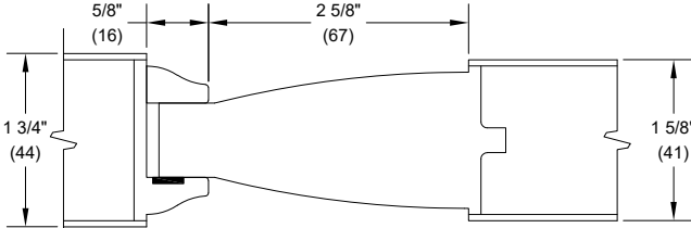
E - Senior Raised
