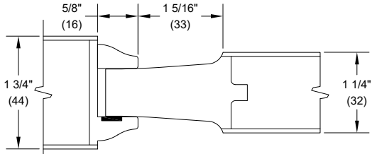
A - Raised
