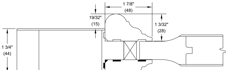
Big Bolection Moulding (BBM)
