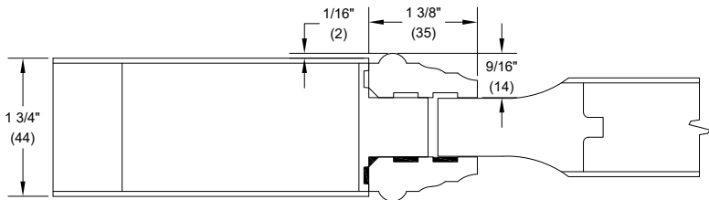
Low Profile Bolection Moulding (LP)
