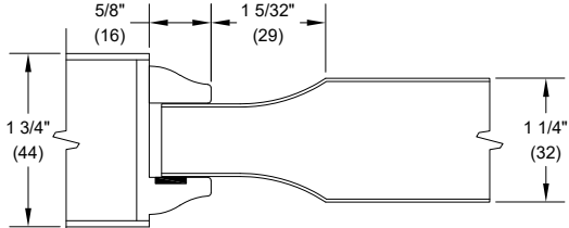
B - Scoop Bladder Pressed
