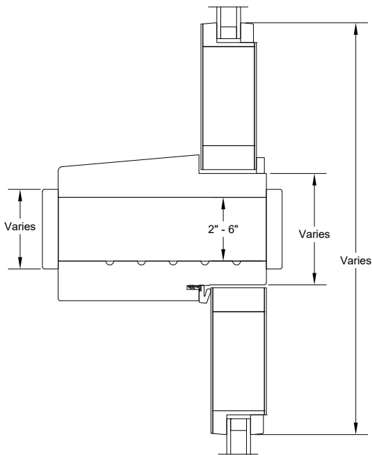
Reinforced Mull
