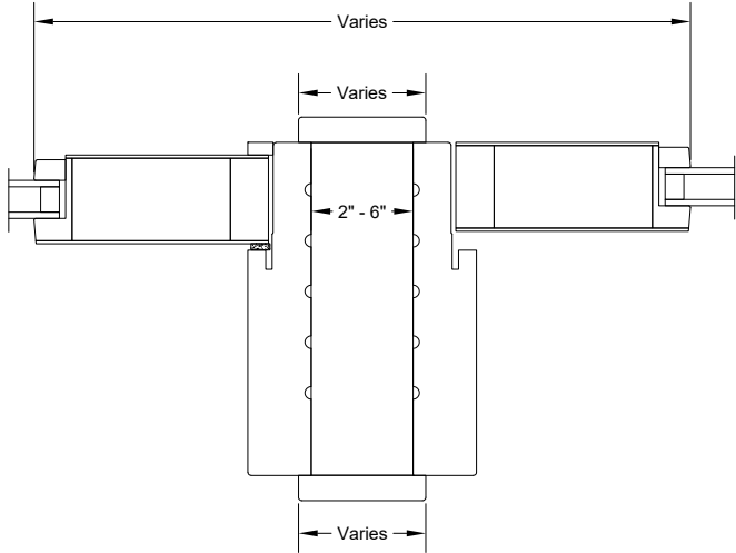
Spread Mull 2" - 6"
