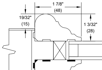
Big Bolection Moulding (BBM)
