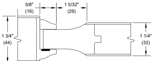
B - Scoop Rim Raised
