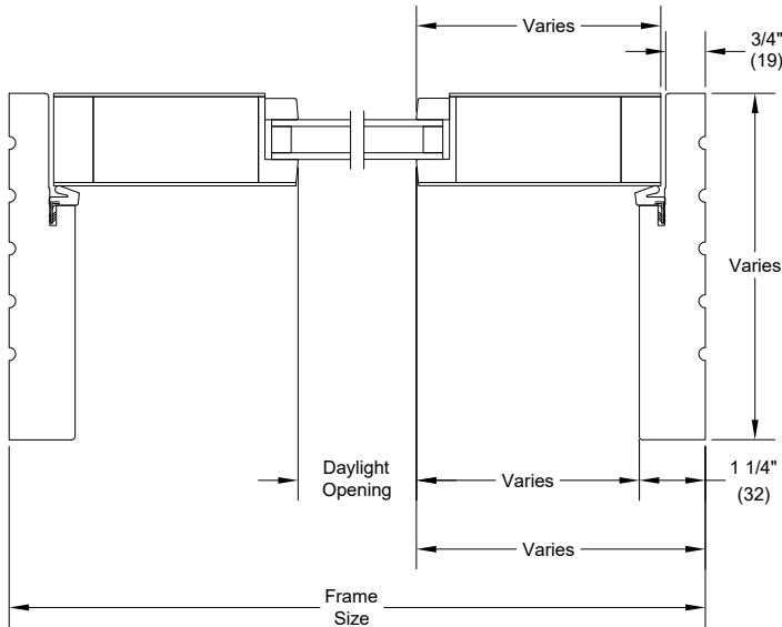
Jambs - Single
