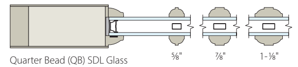
Quarter Bead (QB) SDL Glass
