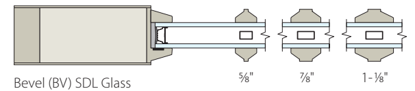
Bevel (BV) SDL Glass
