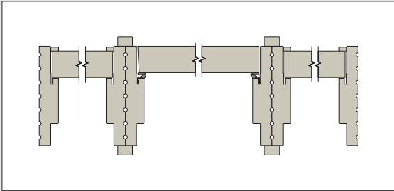
Double Rabbet Frame with Back-to-Back Mull Post
