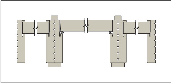
Single Rabbet Frame with Back-to-Back Mull Posts
