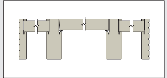
Single Rabbet Frame with 6 3/16\" Uniframe Mull Posts
