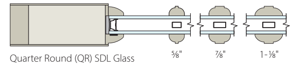
Quarter Round (QR) SDL Glass
